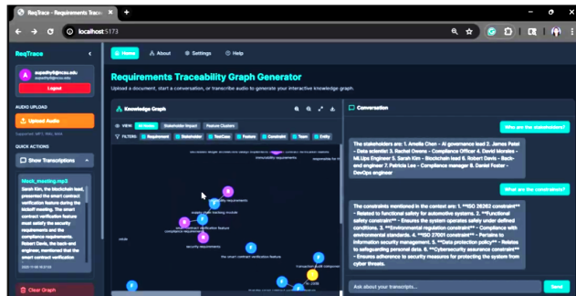
Figure 3.a: ReqTrace: find requirement conflicts.
