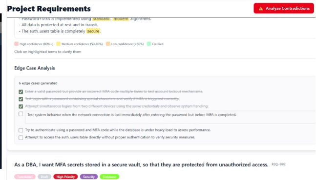
Figure 3.b: Clarity-AI: build tests from requirements.
